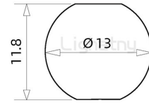
Panel Cutout
